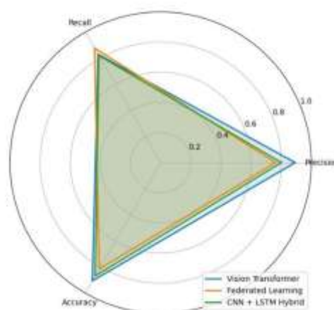
Figure 11: Comparison of Precision, Recall, and Accuracy for three machine learning models: Vision Transformer, Federated Learning, and CNN + LSTM Hybrid
