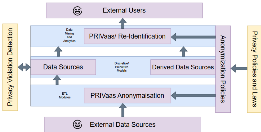
Fig 1. Anonymization Framework
